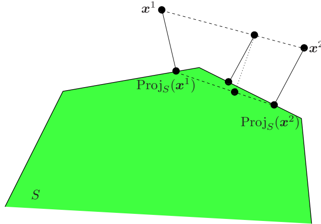
Figure 3.16: The distance function is convex. From the intermediate vector \lambda\mathbf{x}^1 + (1 - \lambda)\mathbf{x}^2 , the distance to the vector \lambda\text{Proj}_S(\mathbf{x}^1) + (1 - \lambda)\text{Proj}_S(\mathbf{x}^2) [the dotted line segment] clearly is longer than the distance to its projection on S [shown as a solid line].
