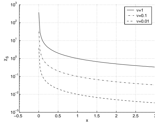
Figure 13.2: The graph of \nu\hat{\chi}_S for various choices of \nu . Note the logarithmic scale.
