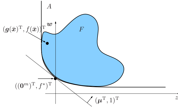
Figure 6.1: Illustration of the set F := \{(\mathbf{g}(\mathbf{x})^T, f(\mathbf{x}))^T \mid \mathbf{x} \in X\} and the set A used in the proof of Theorem 6.9. The idea of the proof is to show that A is convex and that ((\mathbf{0}^m)^T, f^*)^T is not an interior point of A . A hyperplane passing through ((\mathbf{0}^m)^T, f^*)^T and supporting A is used to construct a Lagrange multiplier.
