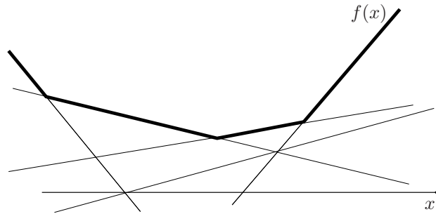
Figure 11.4: A piece-wise affine convex function.
